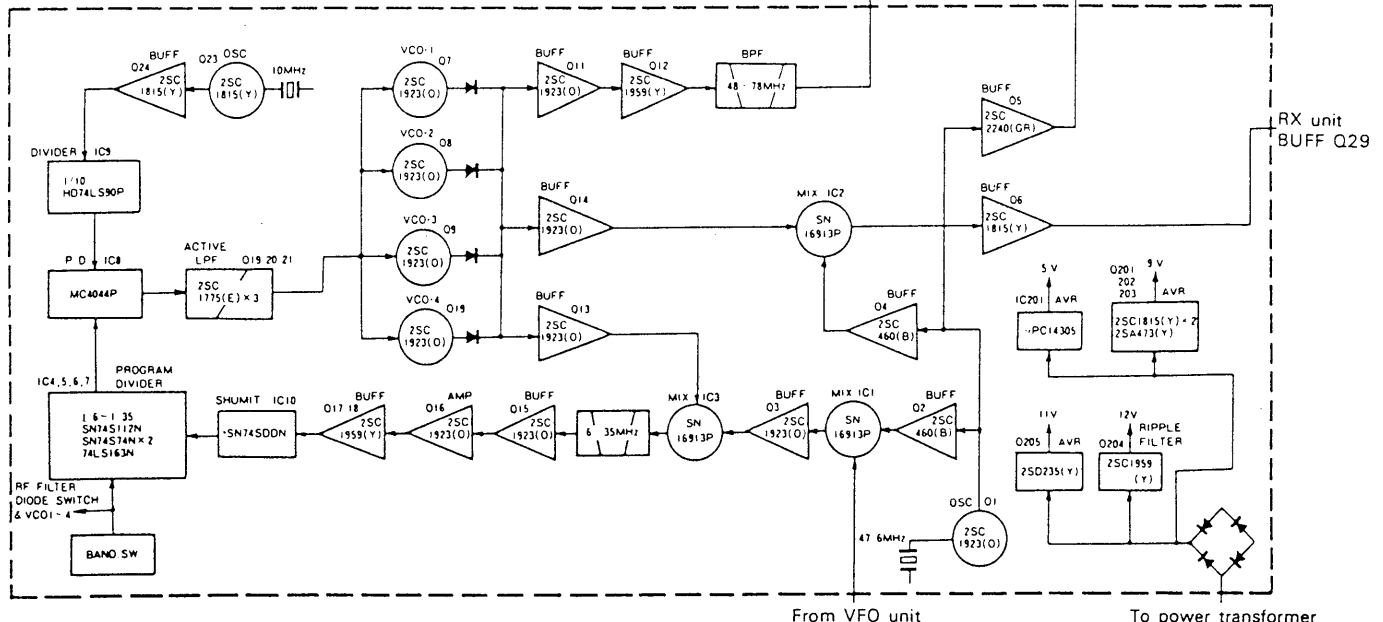
Fig. 1 PLL unit block diagram
